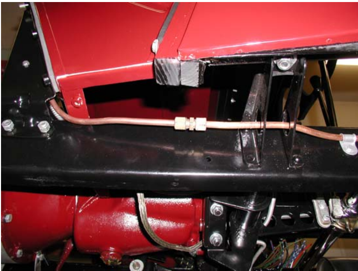
7 – Location of union for fuel line
